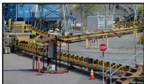
36" Wide x 550' Long Overland Conveyor, 60 HP Electric Motor, Gravity Take-Up..... For Rent or Sale
